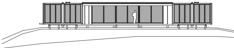
Elevation West
